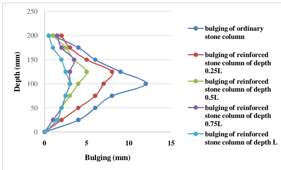
Fig. 24 Bulging of reinforced Stone column of varying depths
