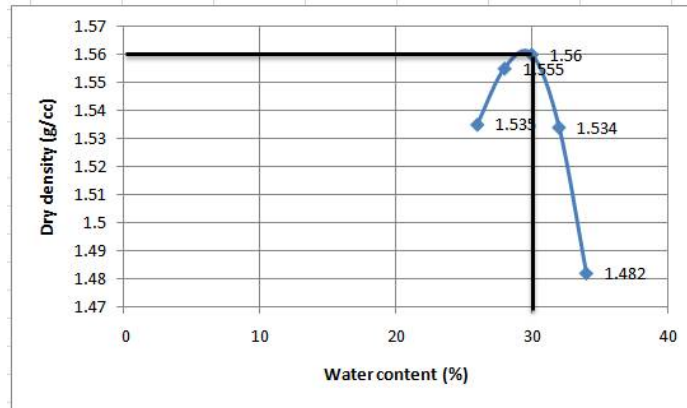
Fig.11 Compaction curve for soft Clay
