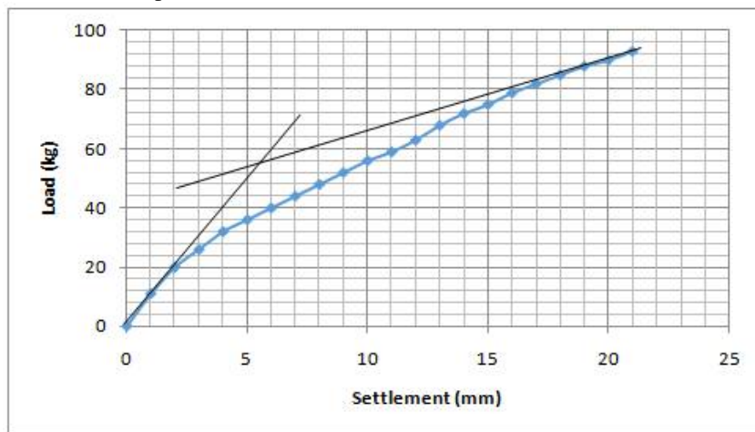
Fig. 15 Load settlement curve of reinforced Stone column with reinforcement depth of 0.5L
