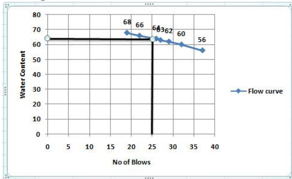
Fig.10 Liquid limit curve for soft Clay
