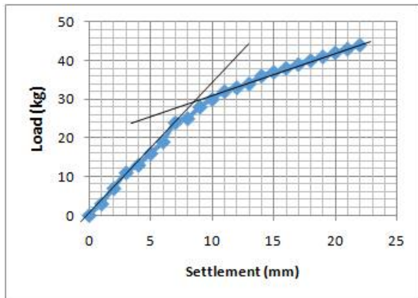
Fig.12 Load-settlement curve of unreinforced Clay bed
