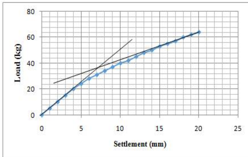
Fig 13 Load-settlement curve of ordinary floating Stone column
