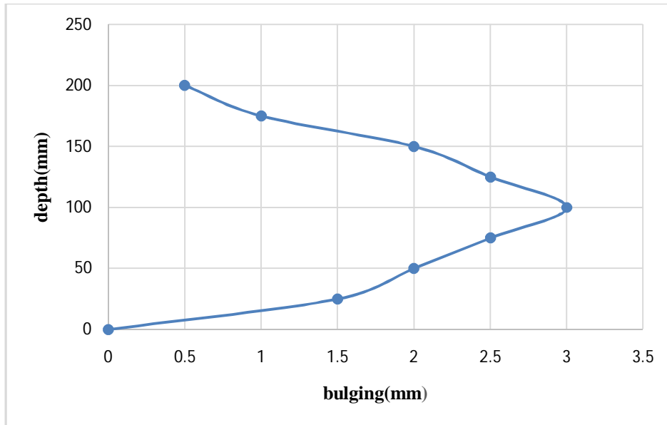
Fig. 23 Bulging curve of reinforced Stone column of L depth
