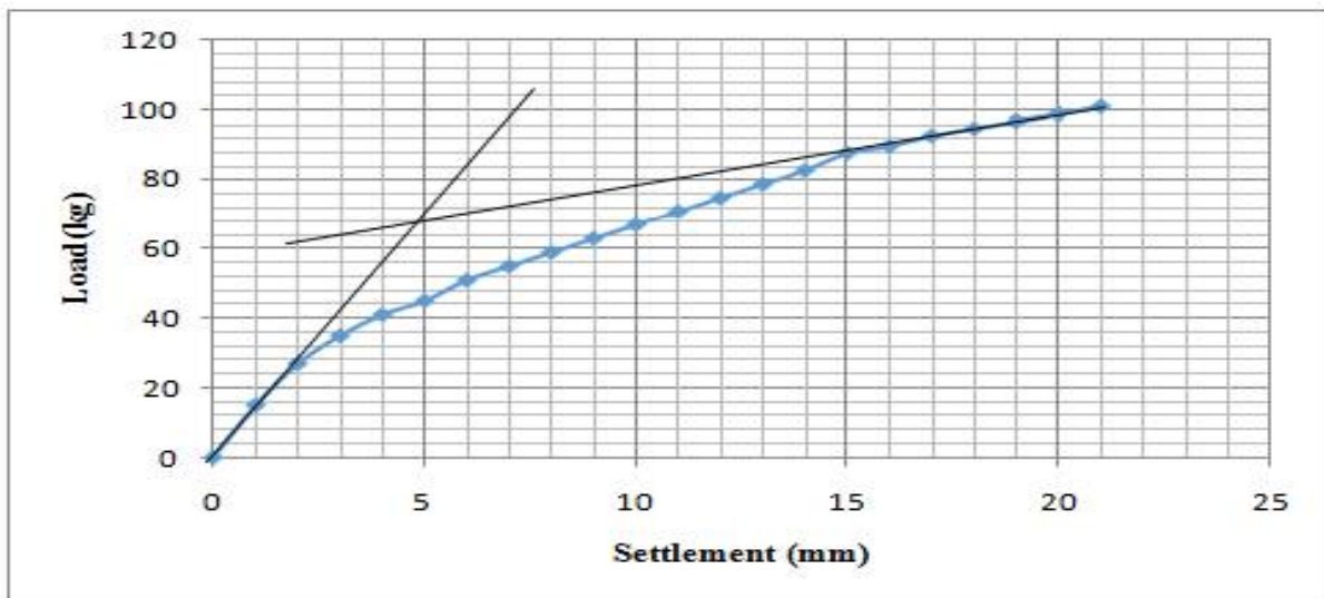
Fig. 16 Load settlement curve of reinforced Stone column with reinforcement depth of 0.75L
