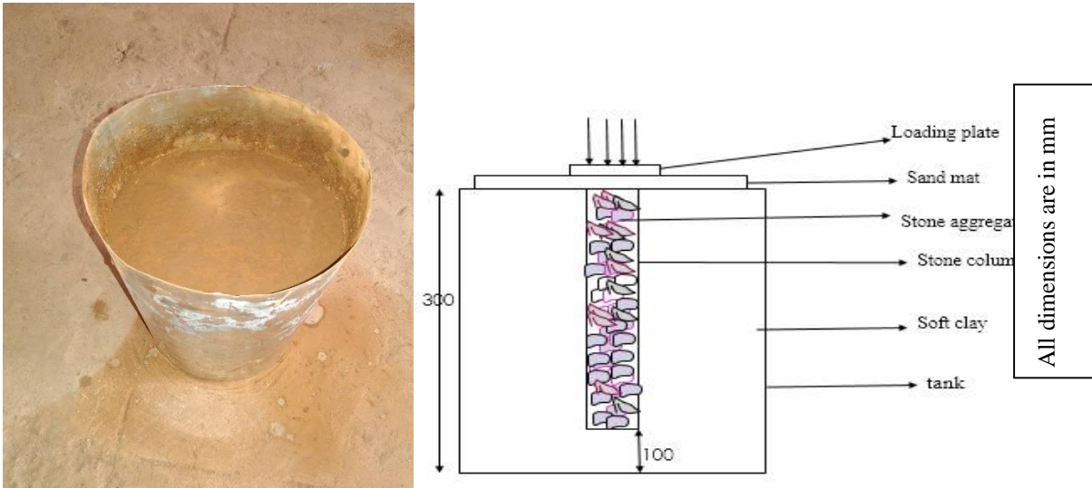
Fig.5 Clay bed Fig.6 Schematic diagram of Stone column
