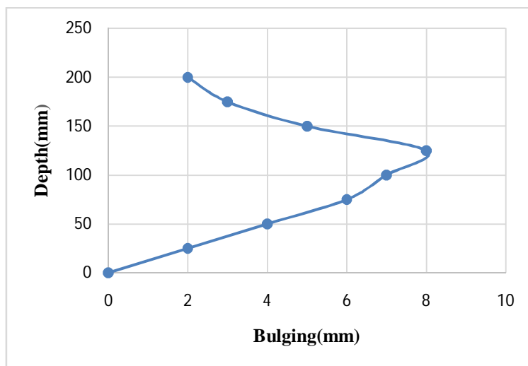
Fig. 20 Bulging curve of reinforced Stone column of 0.25L depth
