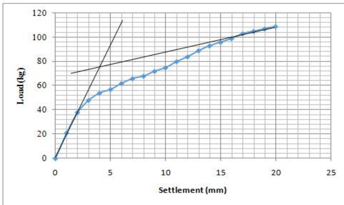
Fig.17 Load settlement curve of reinforced Stone column with reinforcement depth of L
