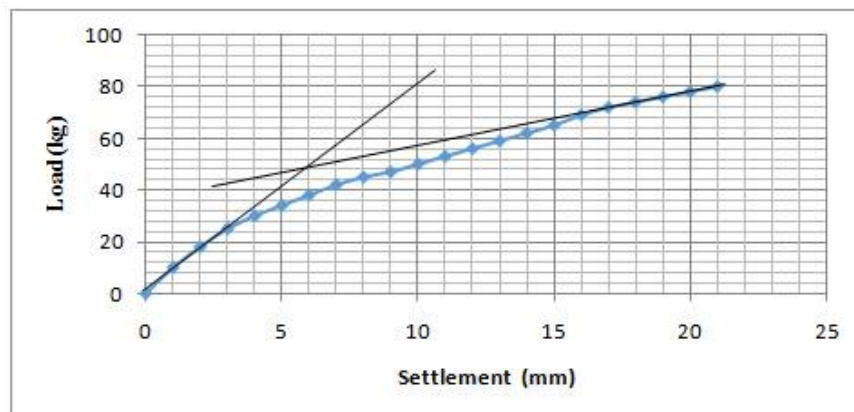
Fig.14 Load settlement curve of reinforced Stone column with reinforcement depth of 0.25L
