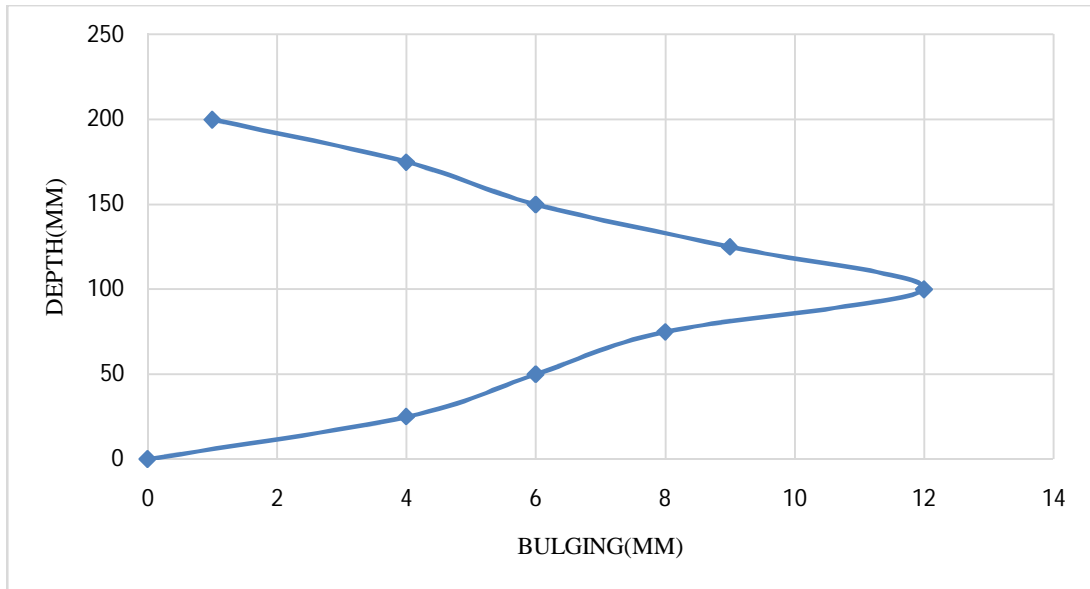
Fig. 19 Bulging curve of ordinary Stone column
