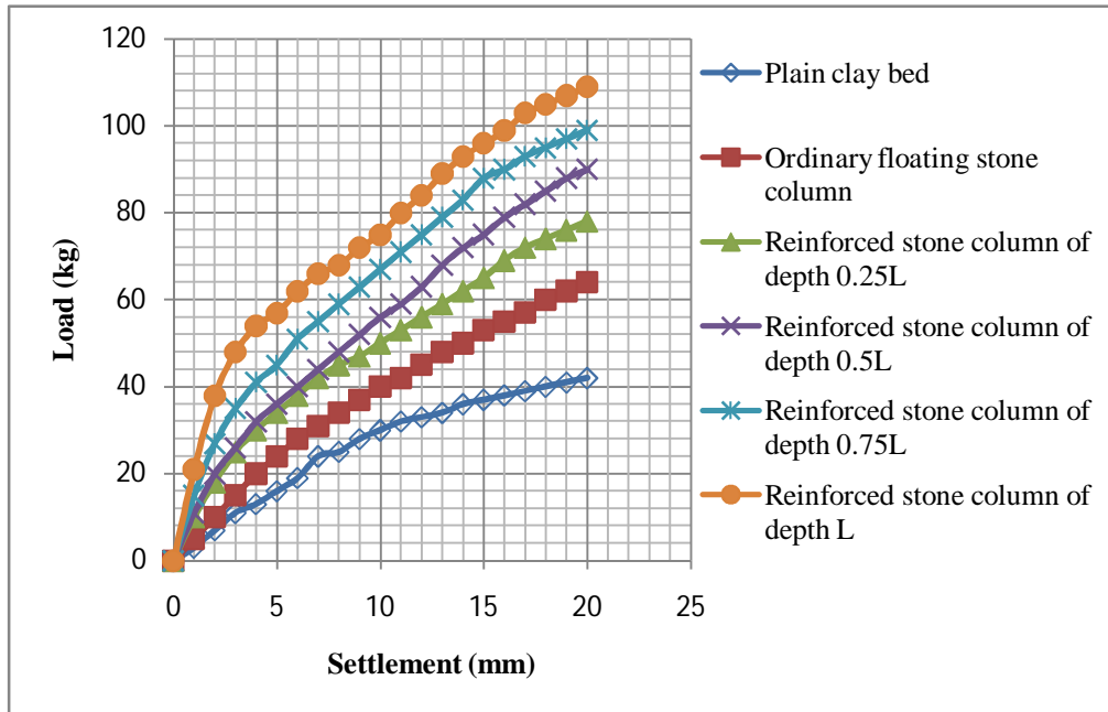
Fig. 18 Load Settlement curves of reinforced Stone columns with varying reinforcement depths.
