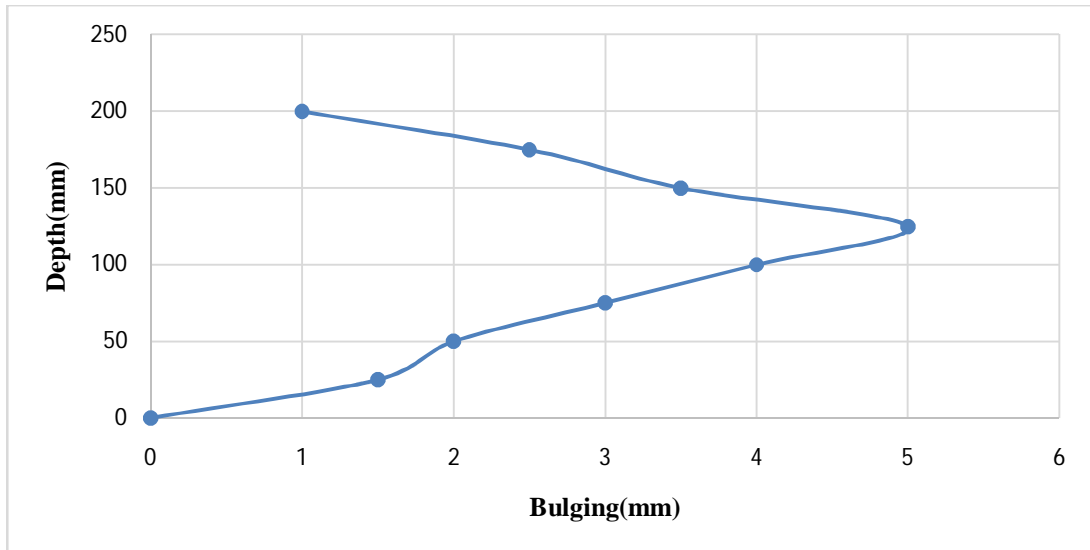
Fig. 21 Bulging curve of reinforced Stone column of 0.5L depth
