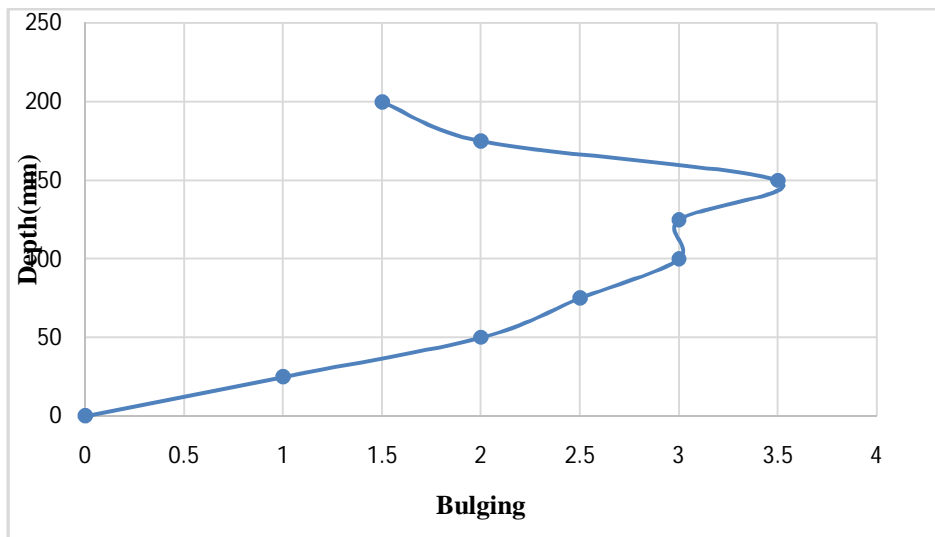
Fig. 22 Bulging curve of reinforced Stone column of 0.75L depth
